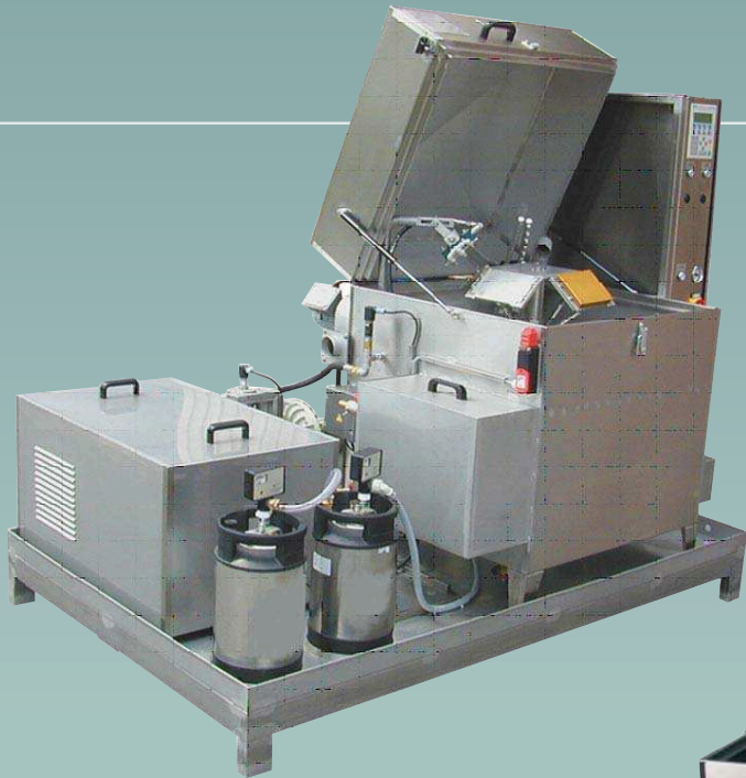
■ type W 80 as special version for high pressure use, rinsing with demineralized water by ion-exchanger, drying with hot air
